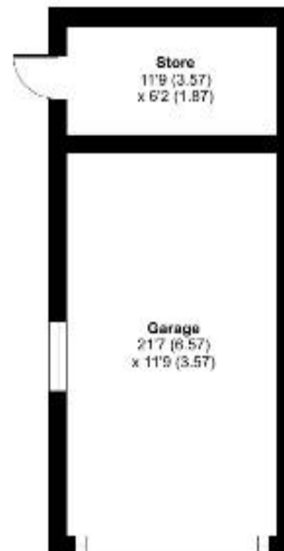
GARAGE / OUTBUILDING 2
